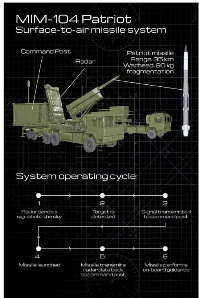
Figure 55. Fakty. How the Patriot air defense system works 110 .
